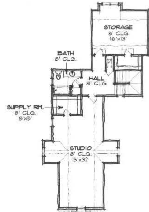
Upper Level Floor Plan 658 S.F. (Upper Level)
