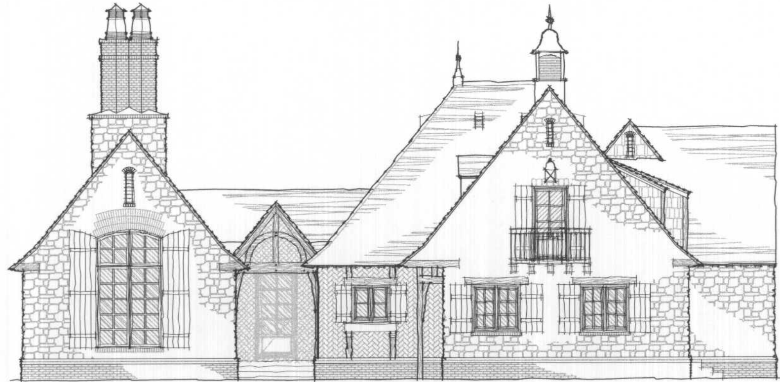
Front Elevation
